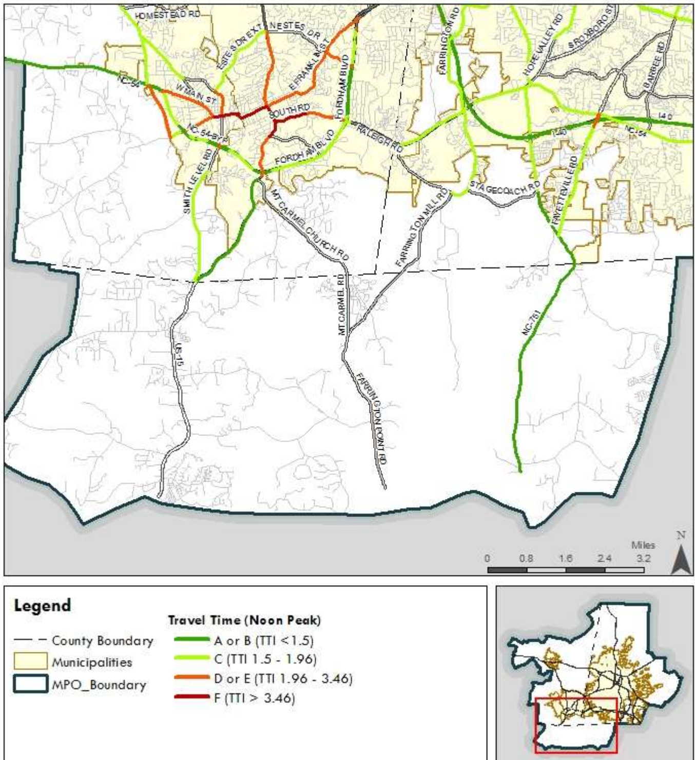
Figure 3-30. Travel Time Index (Noon Peak) - Chatham County
