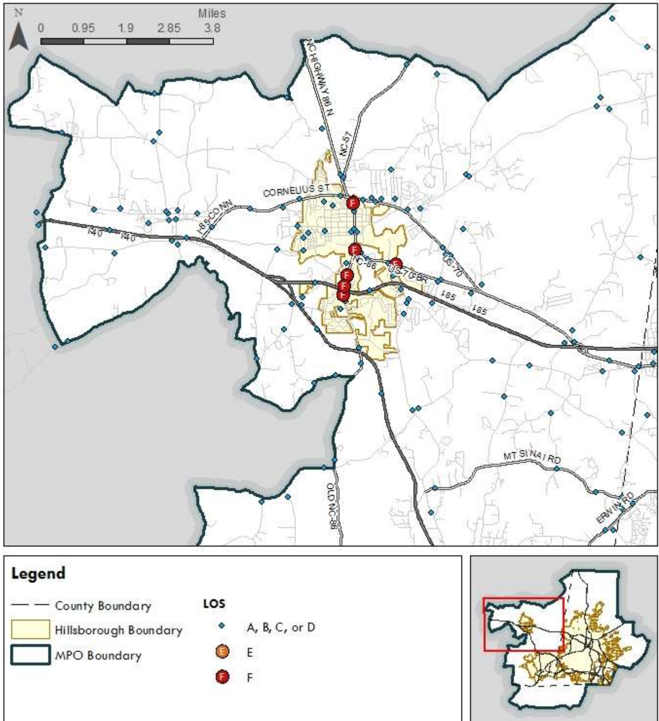
Figure 1-10. 2013 LOS E or F Segments - Hillsborough
