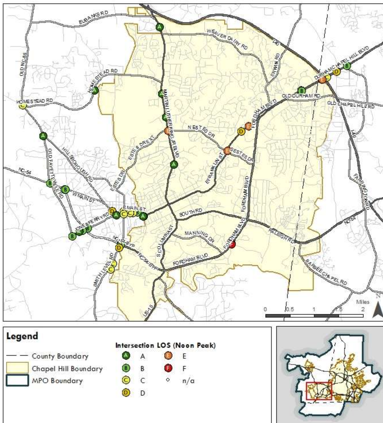
Figure 2-9. Intersection LOS Grades (Noon Peak) - Chapel Hill
