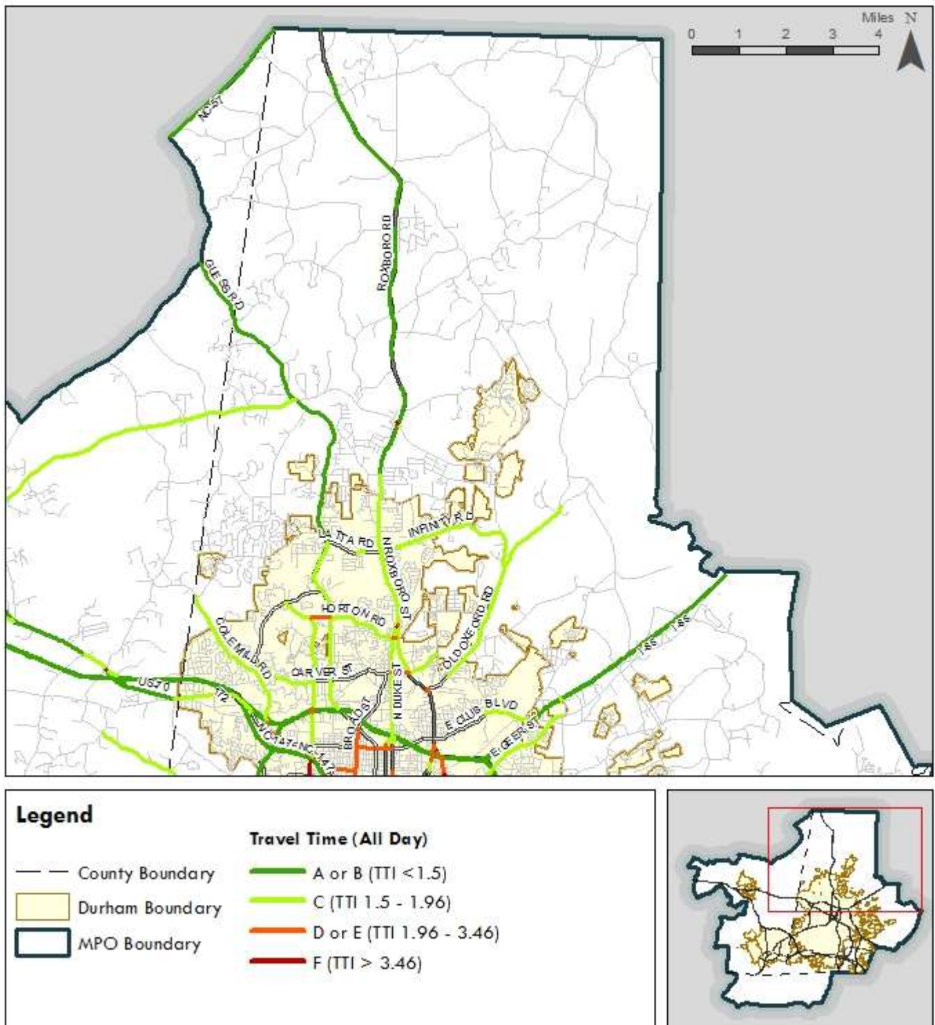
Figure 3-4. Travel Time Index (All Day) - North Durham
