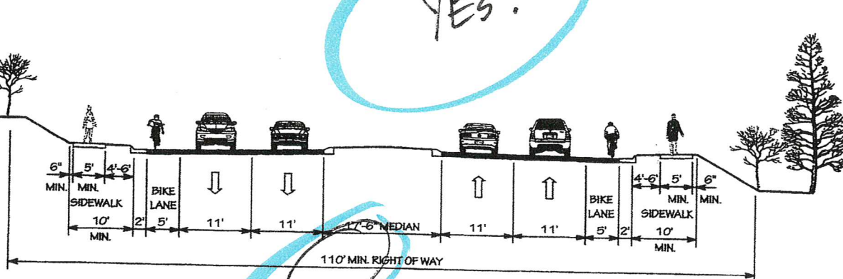
4 LANE DIVIDED (17'-6" RAISED MEDIAN) WITH CURB & GUTTER, BIKE LANES, AND SIDEWALKS POSTED SPEED 35-45 MPH
