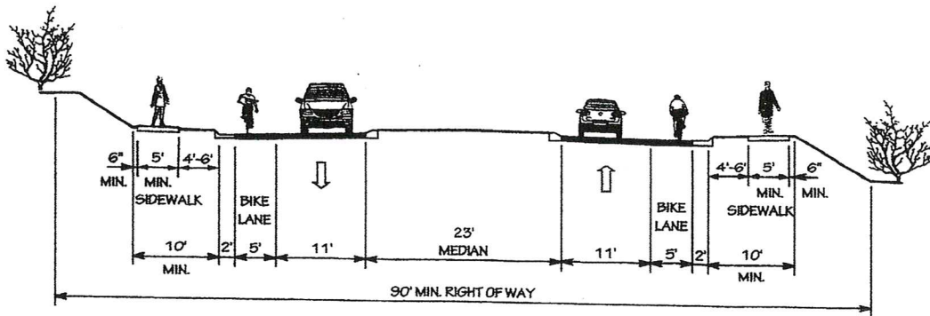
2 LANE DIVIDED (23' RAISED MEDIAN) WITH CURB & GUTTER, BIKE LANES, AND SIDEWALKS POSTED SPEED 25-45 MPH
